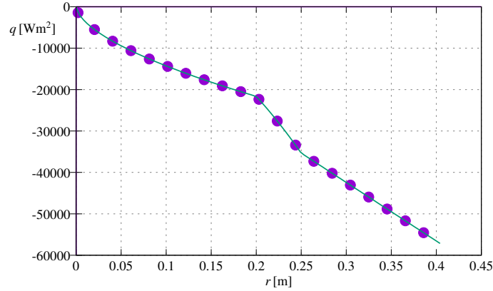
Fig. 6: The plot of function q_r(r, \frac{\pi}{6}) for 0 \leq r \leq R .
