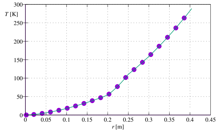
Fig. 4: The plot of function T(r, \frac{\pi}{6}) for 0 \leq r \leq R_0 .
